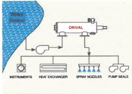
Process Cooling
