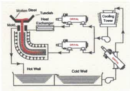
Steel / Continuous Casting
