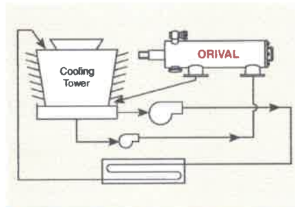
Side Stream w/ Recirculating Pump
